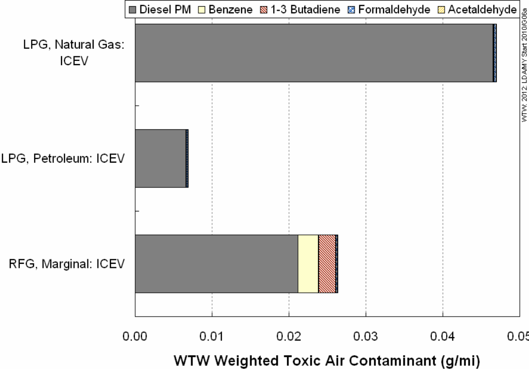
Figure 3-46. Air Toxic Contaminant Emissions for LPG Vehicles (2012 New Vehicle Stock)
