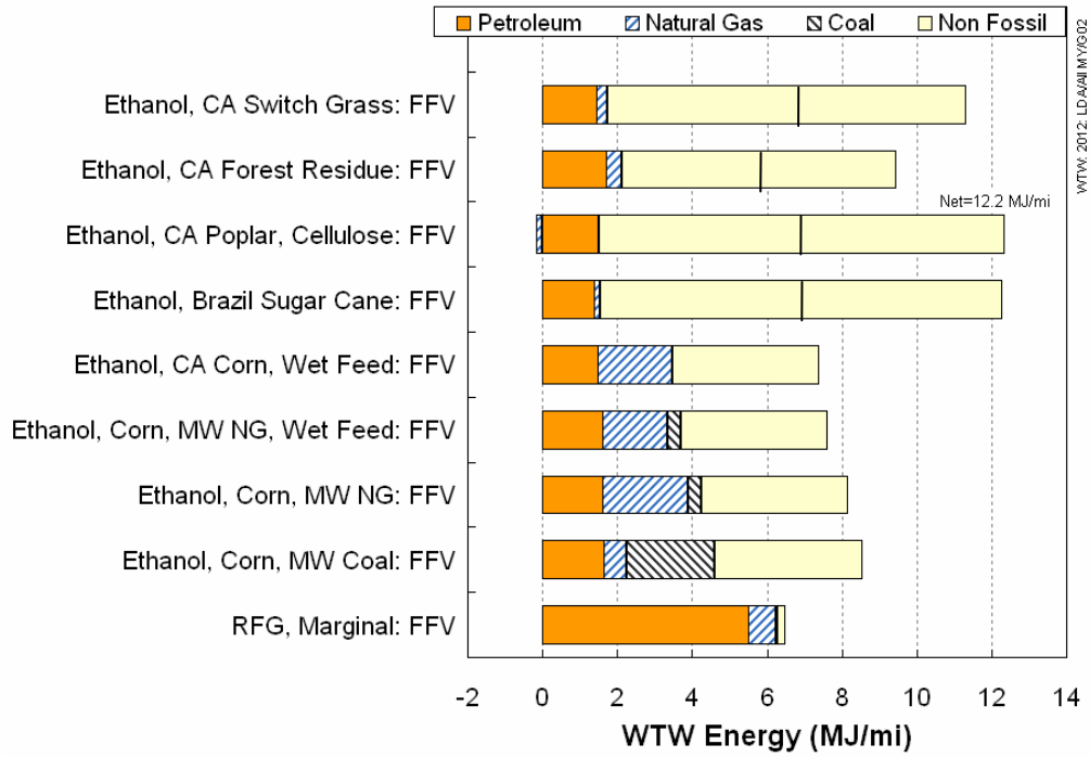
Figure 3-5. WTW Energy Consumption for Ethanol Fuels in Mid-Size Vehicles (2012 Existing Vehicle Stock)
