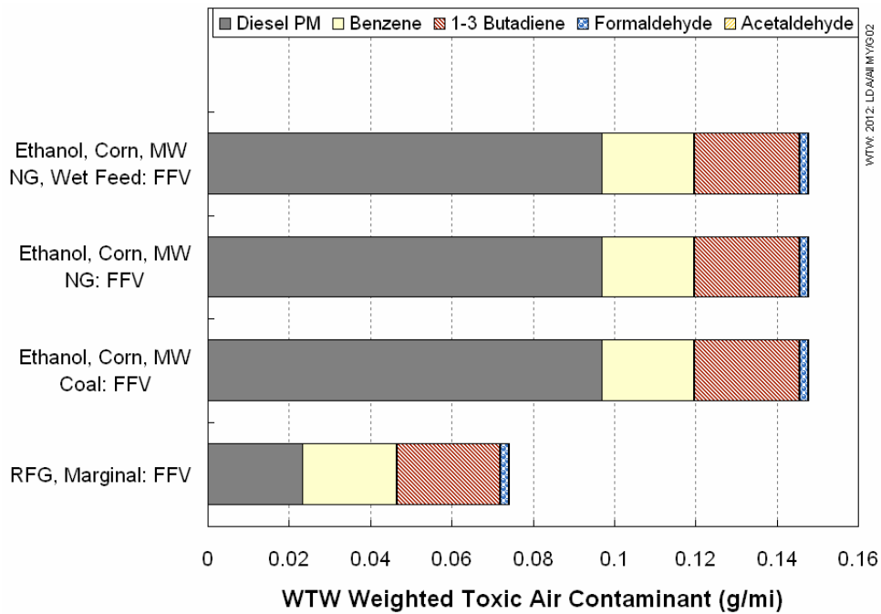
Figure 3-8. Air Toxic Contaminant Emissions for Ethanol Fuels (2012 Existing Vehicle Stock)
