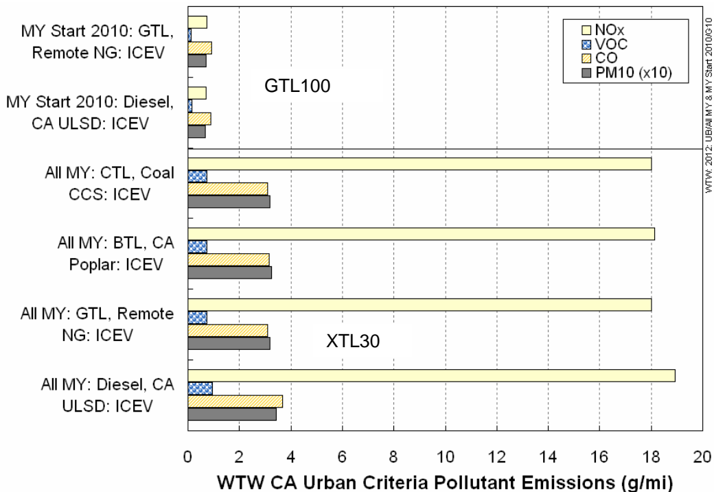
Figure 3-29. Criteria Pollutant Emissions for XTL Urban Buses
