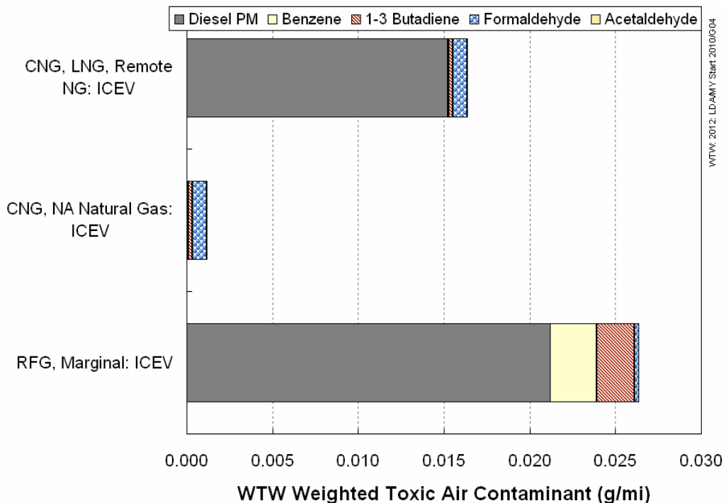
Figure 3-21. Air Toxic Contaminant Emissions for CNG Vehicles (2012 New Vehicle Stock)
