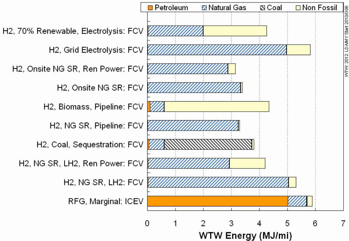
Figure 3-31. WTW Energy Consumption for Hydrogen Midsize Vehicles (2012 New Vehicle Stock)
