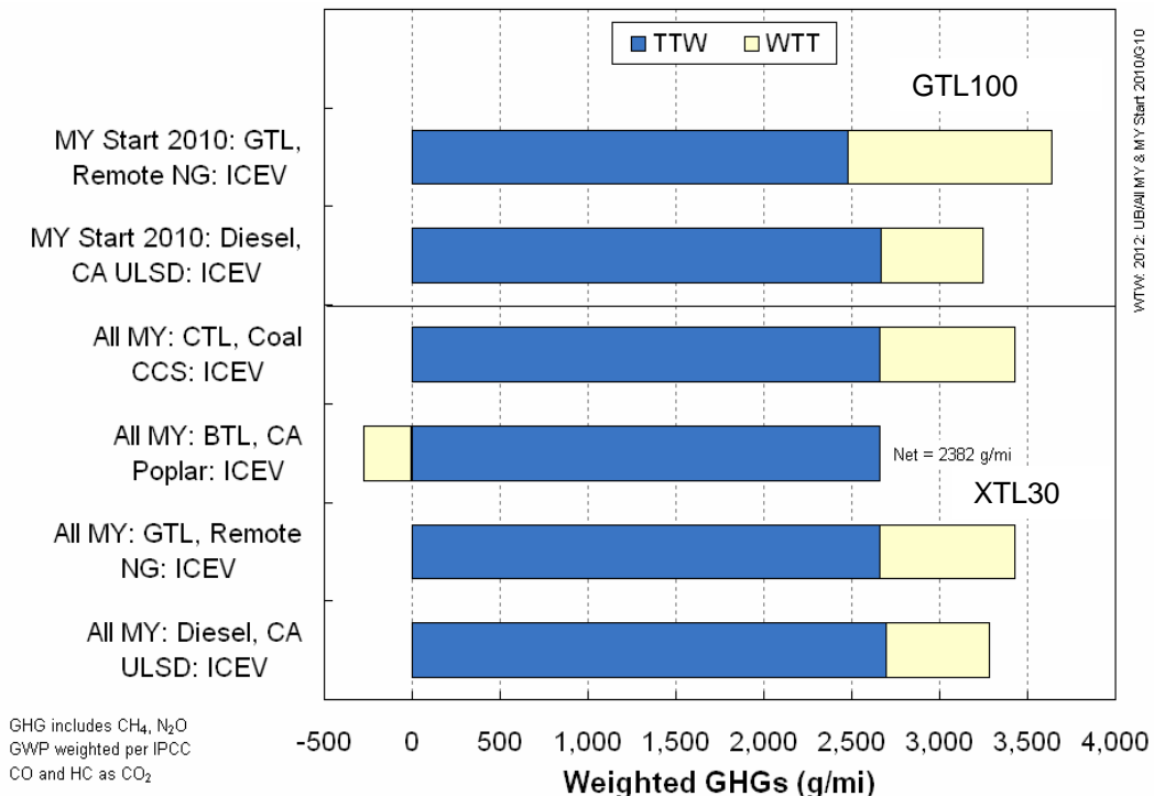
Figure 3-28. WTW GHG Emissions for XTL Urban Buses
