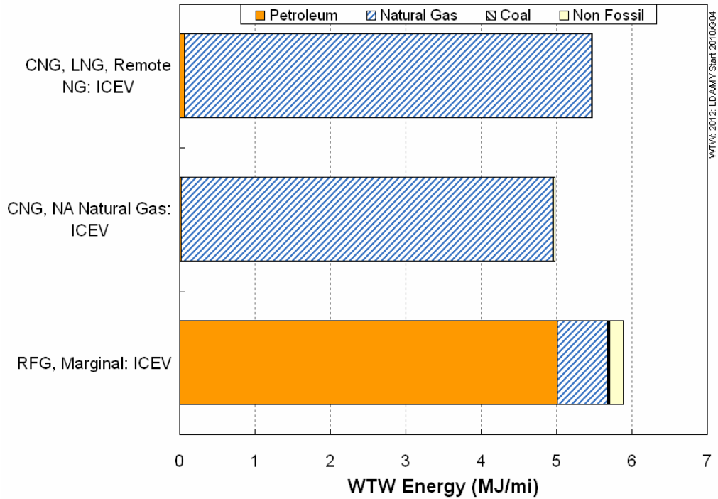
Figure 3-15. WTW Energy Consumption for CNG Midsize Vehicles (2012 New Vehicle Stock)
