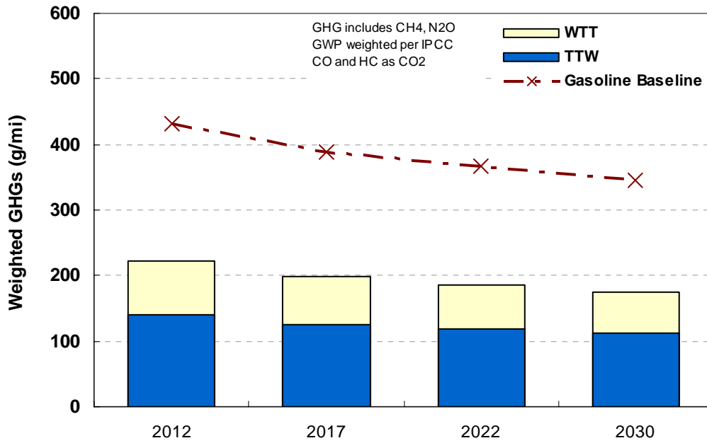
Figure 4-7. WTW GHG Emissions for PHEV Passenger Cars (MY2010 and newer)
