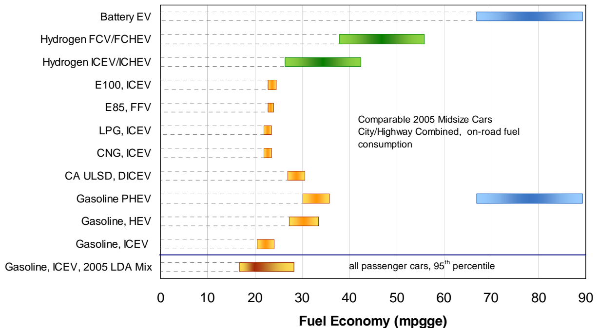
Figure 2-2. Summary of Light-Duty Vehicle Fuel Economies Used in TTW Analysis
