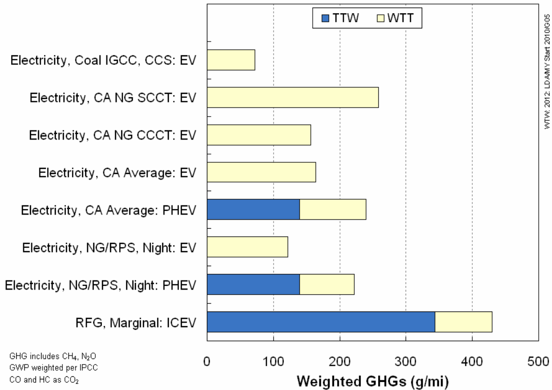
Figure 3-24. WTW GHG Emissions for Electric Vehicles (2012 New Vehicle Stock)
