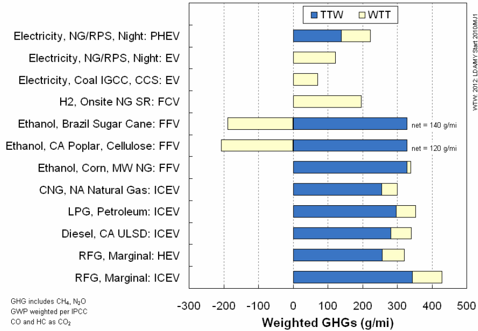
Figure ES-5. 2012 GHG Emissions for Spark Ignited Passenger Car Options (new stock)
