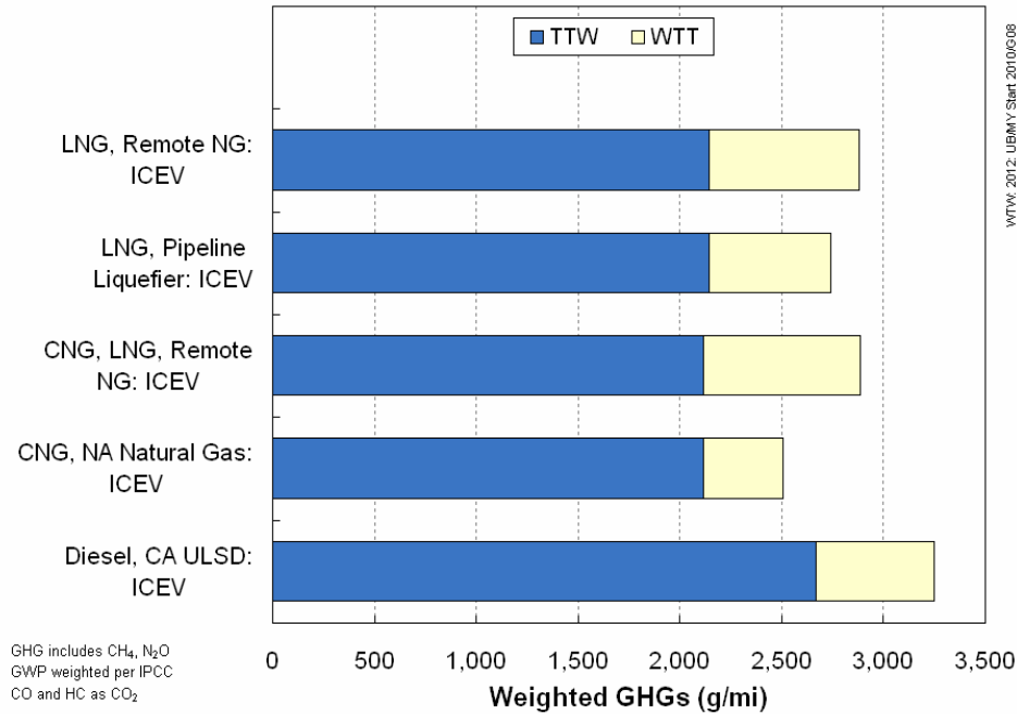
Figure 3-18. WTW GHG Emissions for LNG and CNG Heavy Duty Vehicles (2012 New Vehicle Stock)
