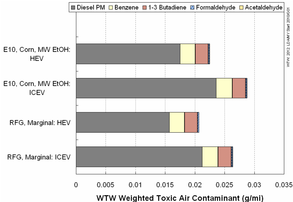
Figure 3-4. WTW Air Toxic Contaminant Emissions for Gasoline Fuels in Mid-Size Vehicles (2012 New Vehicle Stock)
