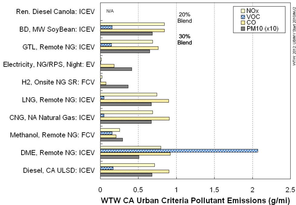
Figure ES-11. 2012 WTW Criteria Pollutant Emissions from Urban Buses (new stock)
