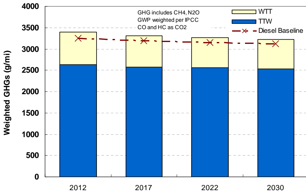
Figure 4-8. WTW GHG Emissions for Natural Gas Derived FTD30 Buses (MY2010 and newer)
