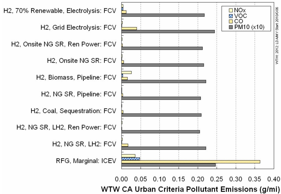
Figure 3-35. Criteria Pollutant Emissions for Midsize Hydrogen Vehicles (2012 New Vehicle Stock)
