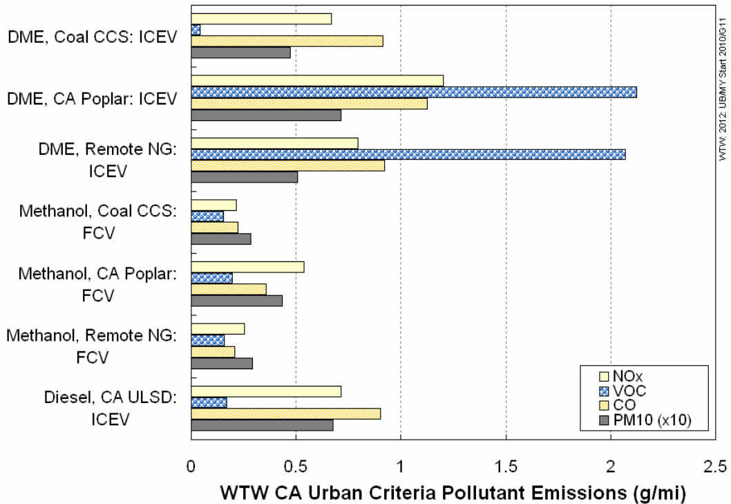
Figure 3-41. Criteria Pollutant Emissions for Synthetic Fuel Vehicles (2012 New Stock)
