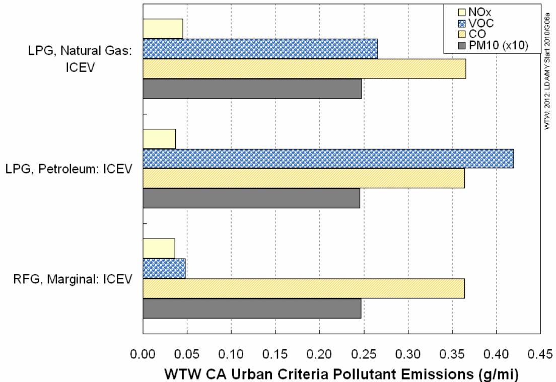
Figure 3-45. Criteria Pollutant Emissions for LPG Vehicles (2012 New Vehicle Stock)
