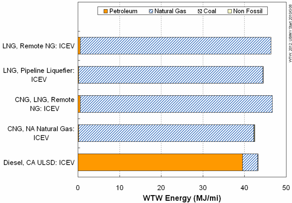
Figure 3-17. WTW Energy Consumption for LNG and CNG Heavy Duty Vehicles (2012 New Vehicle Stock)
