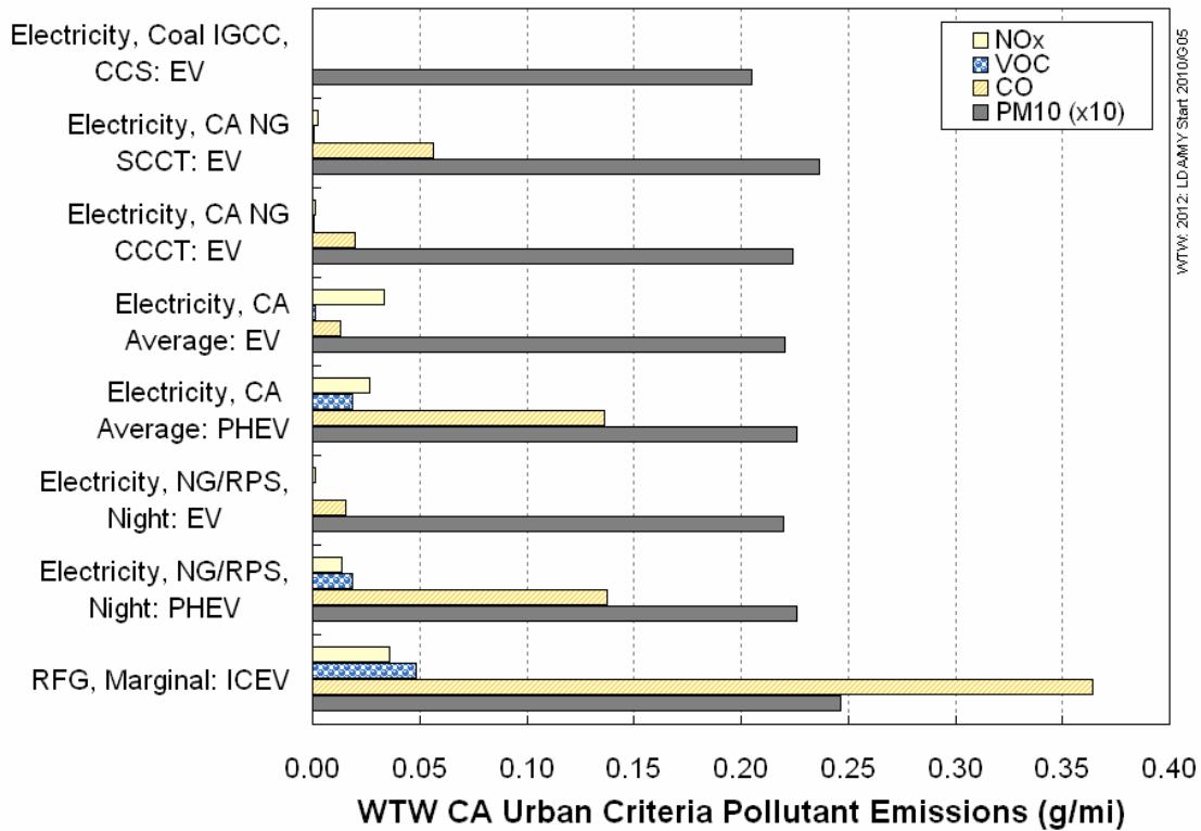
Figure 3-25. Criteria Pollutant Emissions for Midsize Electric Vehicles (2012 New Vehicle Stock)
