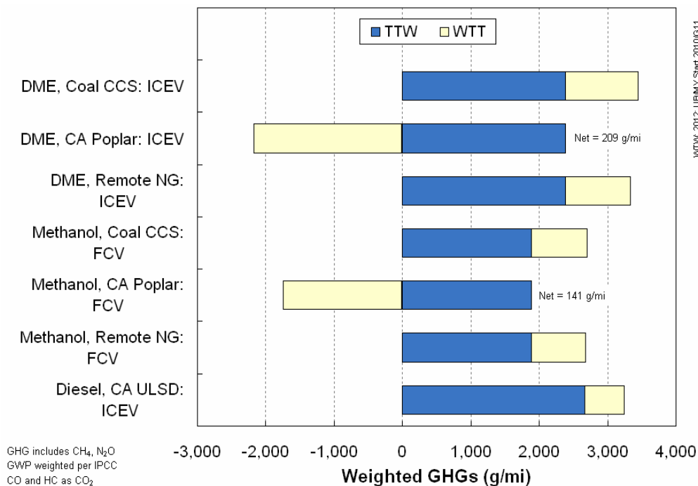
Figure 3-40. WTW GHG Emissions for Synthetic Fuel Vehicles (2012 New Stock)
