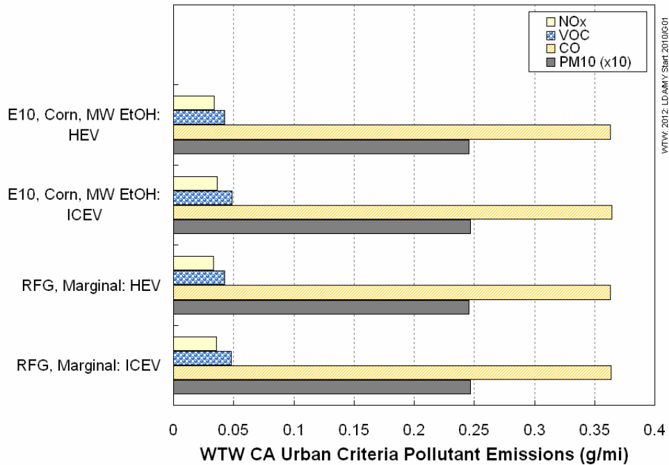
Figure 3-3. WTW Criteria Pollutant Emissions for Gasoline Fuels in Mid-Size Vehicles (2012 New Vehicle Stock)
