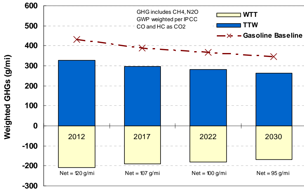
Figure 4-5. WTW GHG Emissions for Biomass Based E-85 Passenger Cars (MY2010 and newer)
