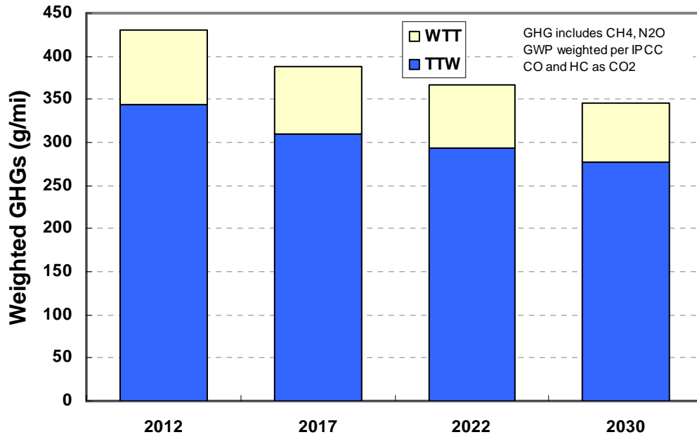
Figure 4-3. WTW GHG Emissions for Gasoline Passenger Cars (MY2010 and newer)
