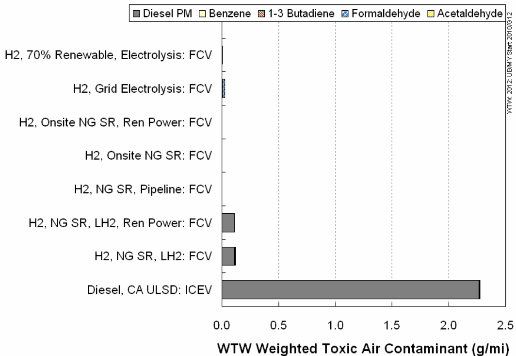
Figure 3-38. Air Toxic Emissions for Hydrogen Urban Buses (2012 New Vehicle Stock)
