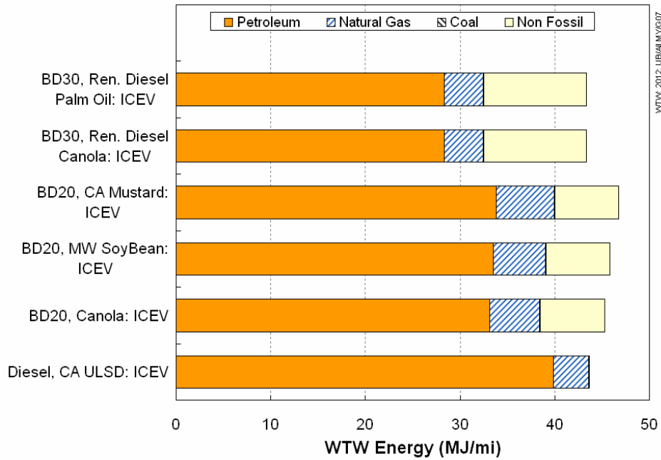
Figure 3-10. WTW Energy Consumption for Bio and Renewable Diesel Fueled Urban Buses (2012 Existing Vehicle Stock)
