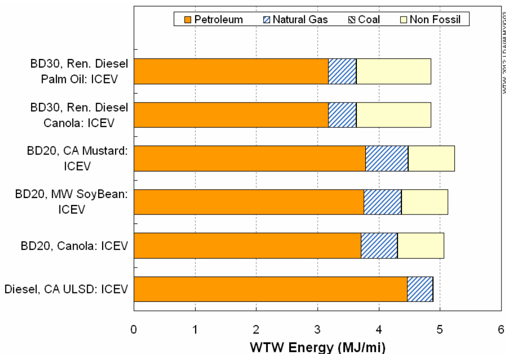
Figure 3-9. WTW Energy Consumption for Bio and Renewable Diesel Fueled Midsize Vehicles (2012 Existing Vehicle Stock)
