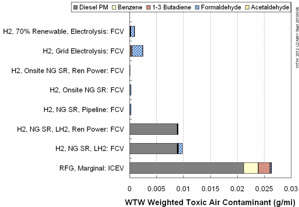
Figure 3-37. Air Toxic Emissions for Midsize Hydrogen Vehicles (2012 New Vehicle Stock)
