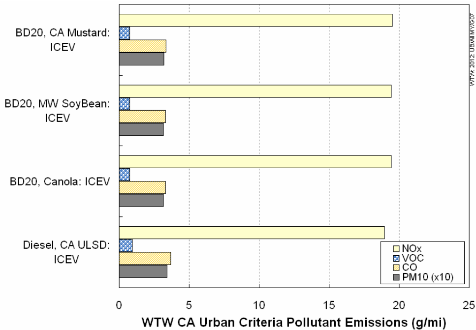
Figure 3-14. Criteria Pollutant Emissions for Bio and Renewable Diesel Fueled Urban Buses (2012 Existing Vehicle Stock)
