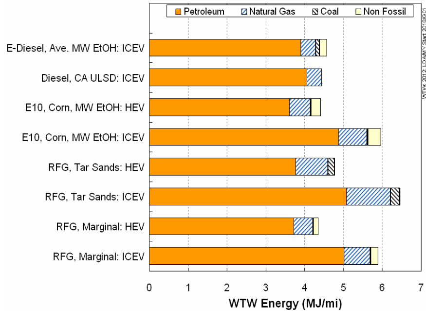
Figure 3-1. WTW Energy Consumption for Petroleum Fuels in Mid-Size Vehicles (2012 New Vehicle Stock)
