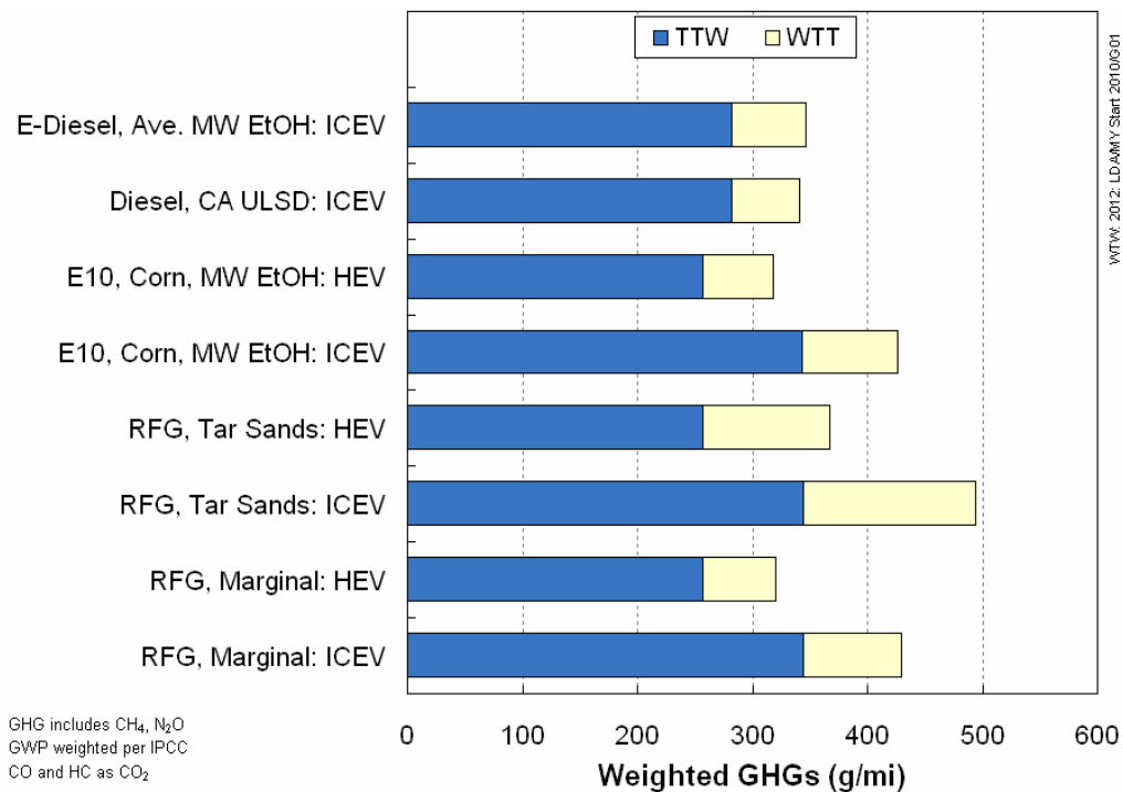
Figure 3-2. WTW GHG Emissions for Petroleum Fuels in Mid-Size Vehicles (2012 New Vehicle Stock)
