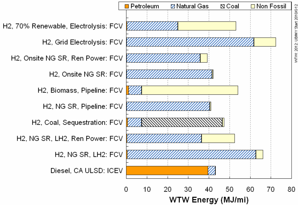
Figure 3-32. WTW Energy Consumption for Hydrogen Urban Buses (2012 New Vehicle Stock)
