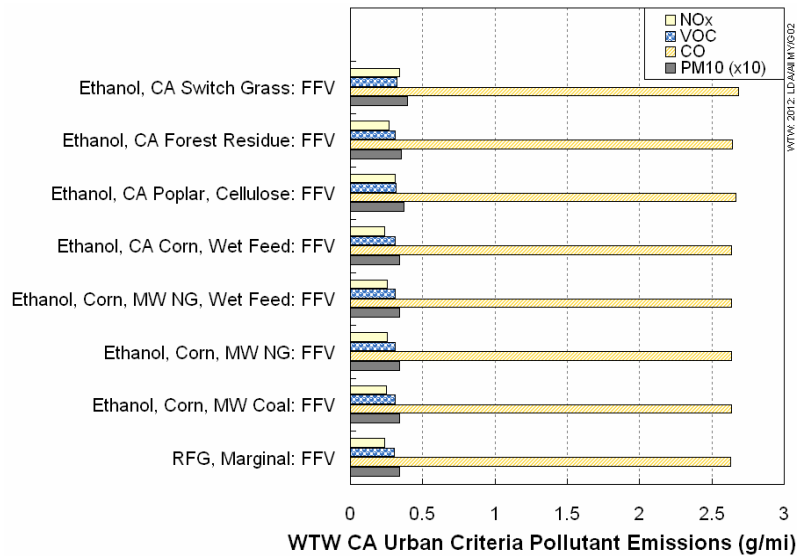
Figure 3-7. Criteria Pollutant Emissions for Ethanol Fuels (2012 Existing Vehicle Stock)
