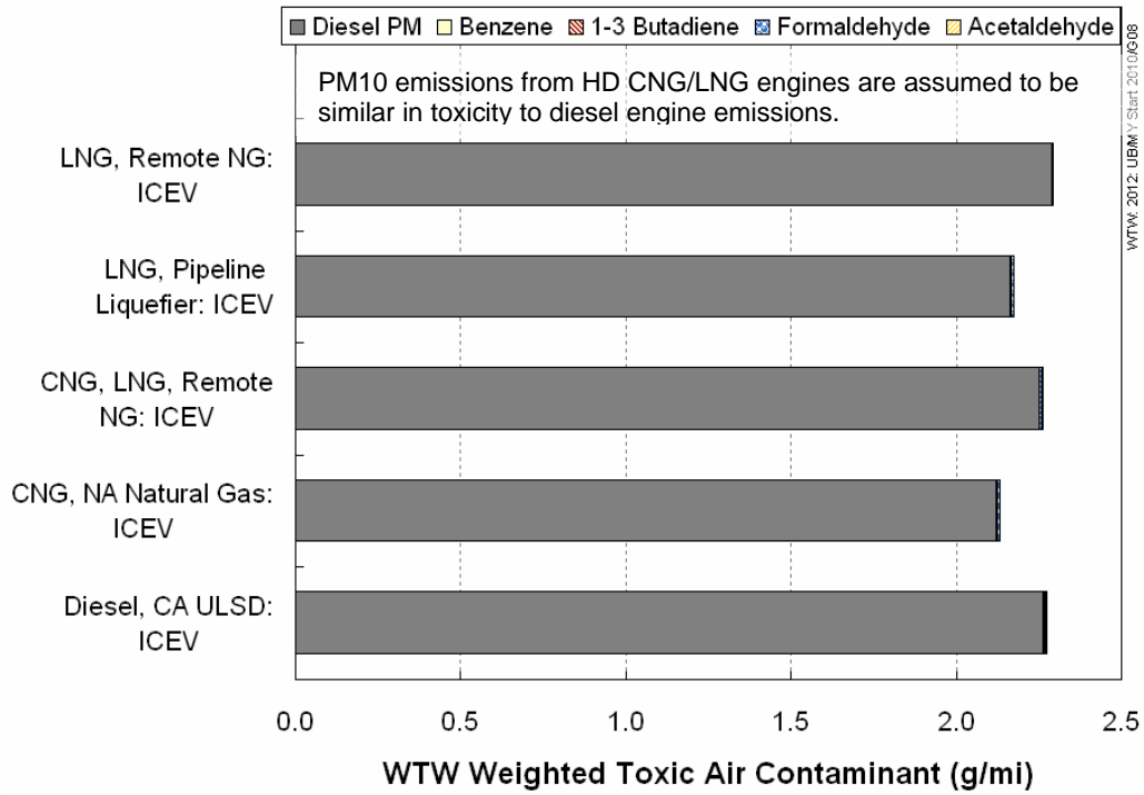
Figure 3-22. Air Toxic Contaminant Emissions for LNG and CNG Urban Buses (2012 New Vehicle Stock)
