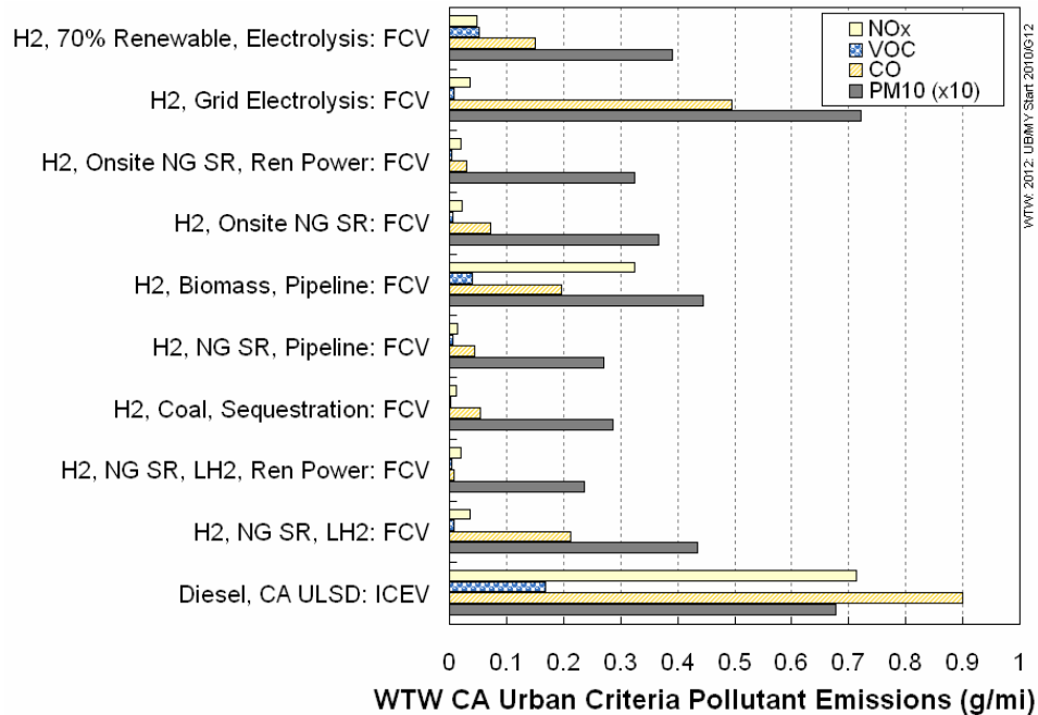
Figure 3-36. Criteria Pollutant Emissions for Hydrogen Urban Buses (2012 New Vehicle Stock)
