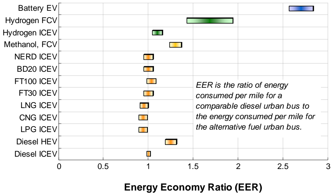
Figure ES-4. Summary of Urban Bus EERs Utilized in TTW Analysis
