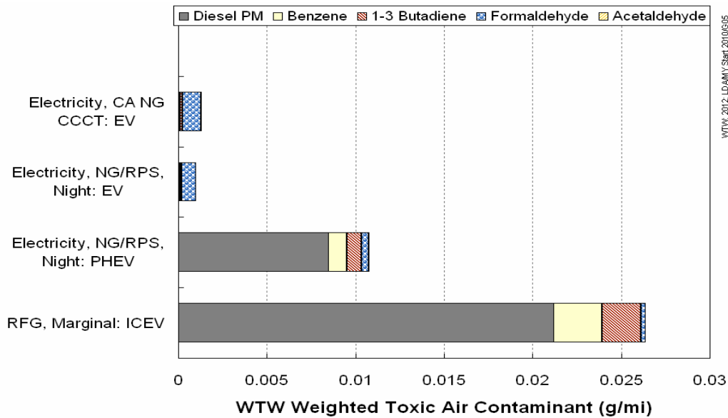
Figure 3-26. Air Toxic Emissions for Midsize Electric Vehicles (2012 New Vehicle Stock)
