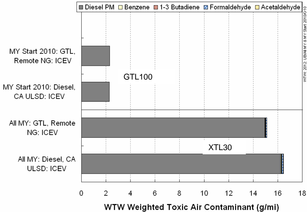
Figure 3-30. Air Toxic Contaminant Emissions for XTL Urban Buses
