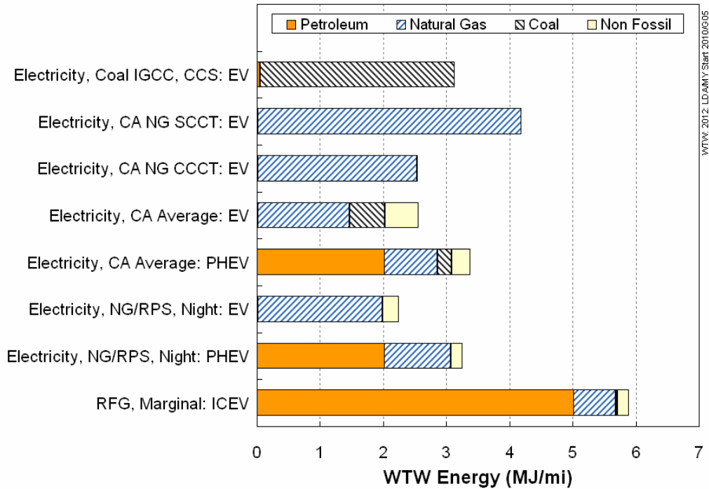
Figure 3-23. WTW Energy Consumption for Midsize Electric Vehicles (2012 New Vehicle Stock)
