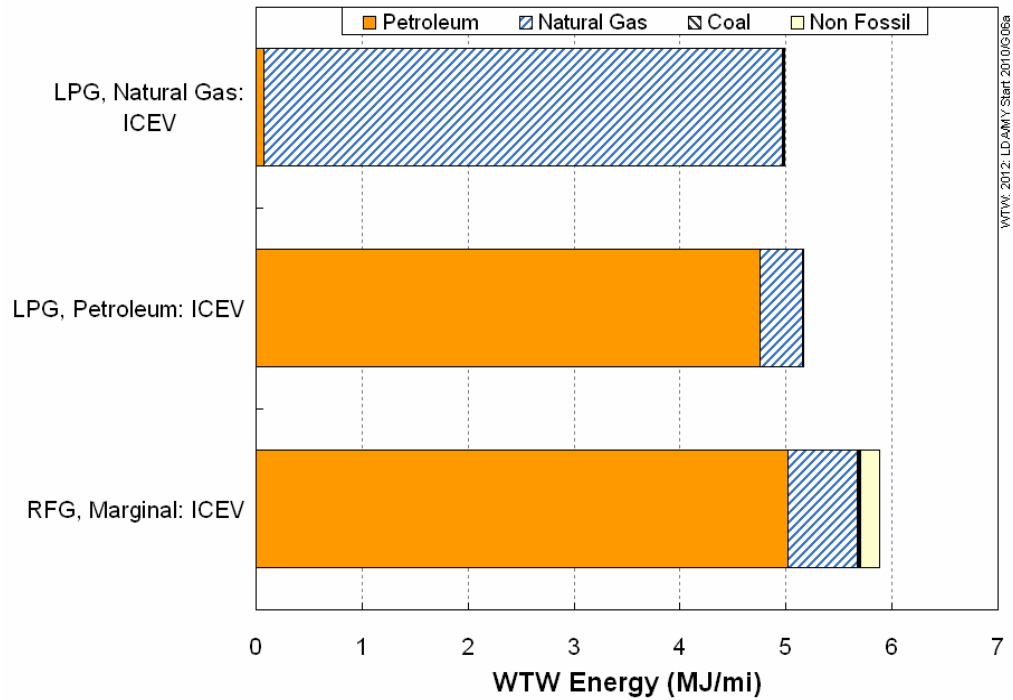
Figure 3-43. WTW Energy Consumption for LPG Vehicles (2012 New Vehicle Stock)
