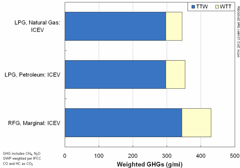
Figure 3-44. WTW GHG Emissions for LPG Vehicles (2012 New Vehicle Stock)
