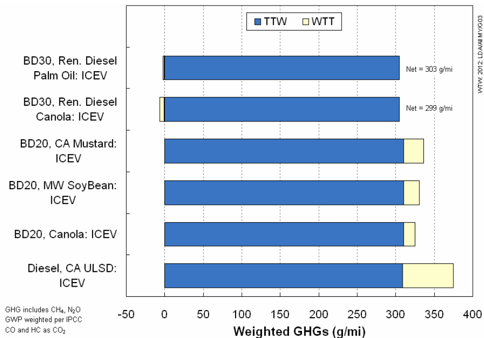
Figure 3-11. WTW GHG Emissions for Bio and Renewable Diesel Fueled Midsize Vehicles (2012 Existing Vehicle Stock)
